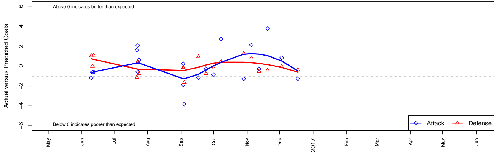
Pumas UNAM B03 Dots are actual minus expected GF (blue circles) and GA (red triangles). Blue line is smoothed change in attack strength. Red is smoothed change in defense strength.
